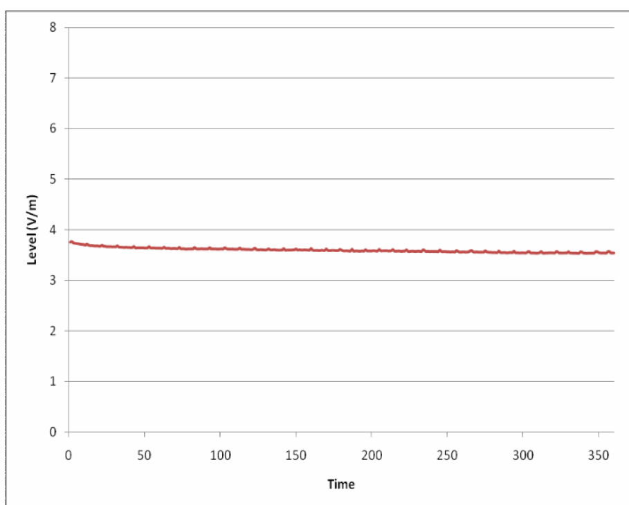
Electric field strengths recorded over 6 min period using 3 GHz probe at point of max NIR:
